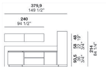
pensili / basi wall units / base units
